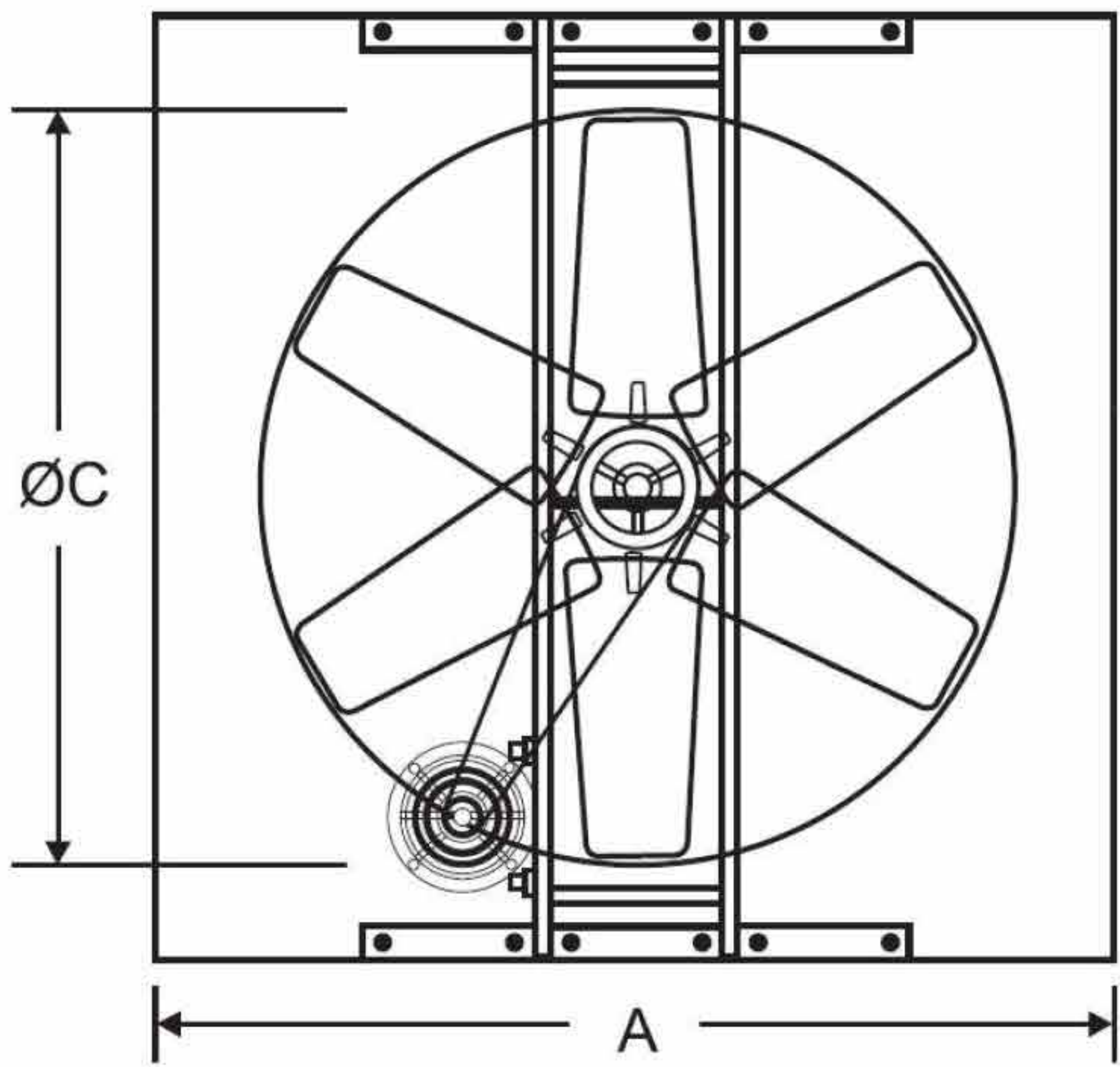
VISTA TRASERA (BACK VIEW)
