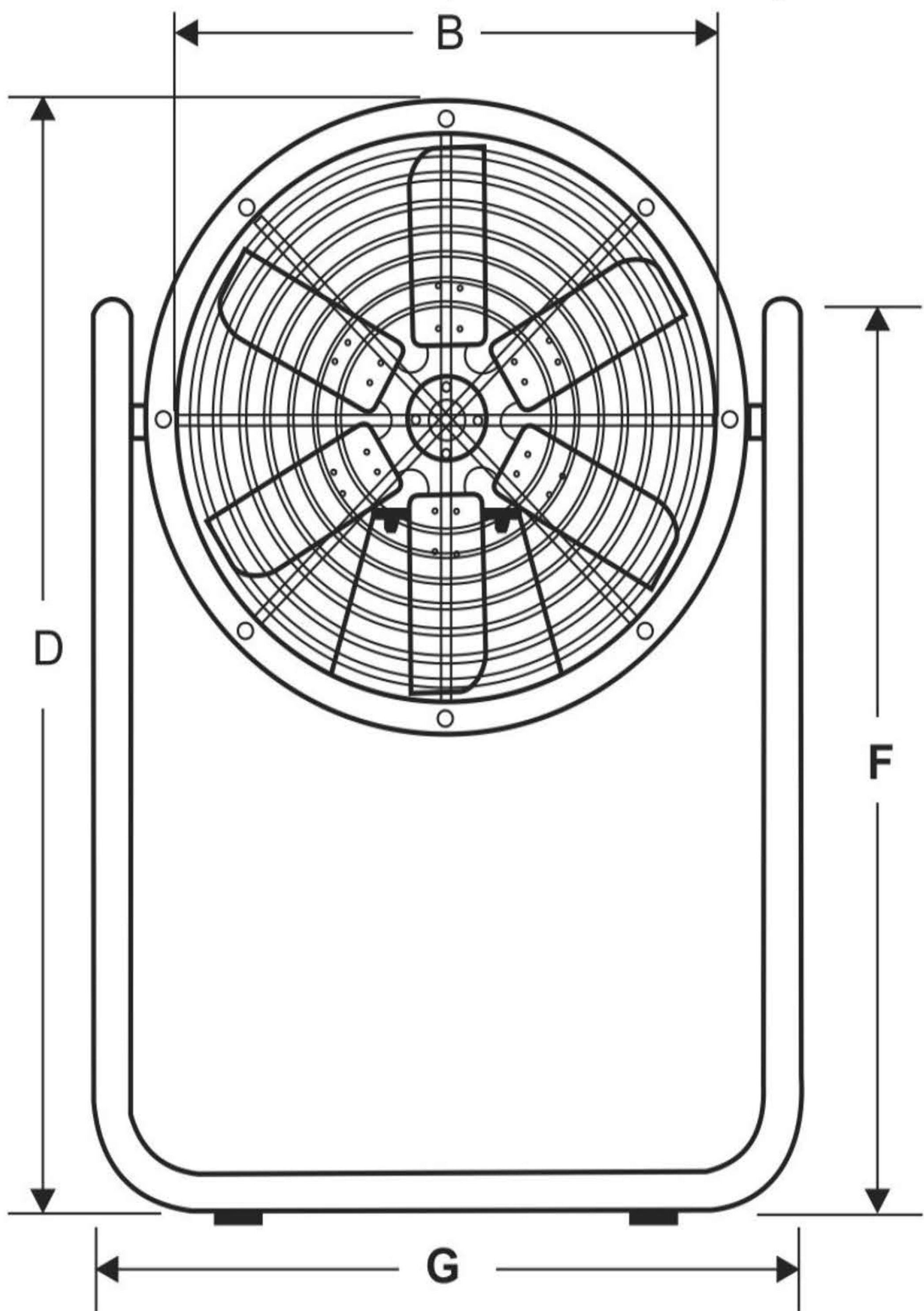
Vista Frontal (Front View)
