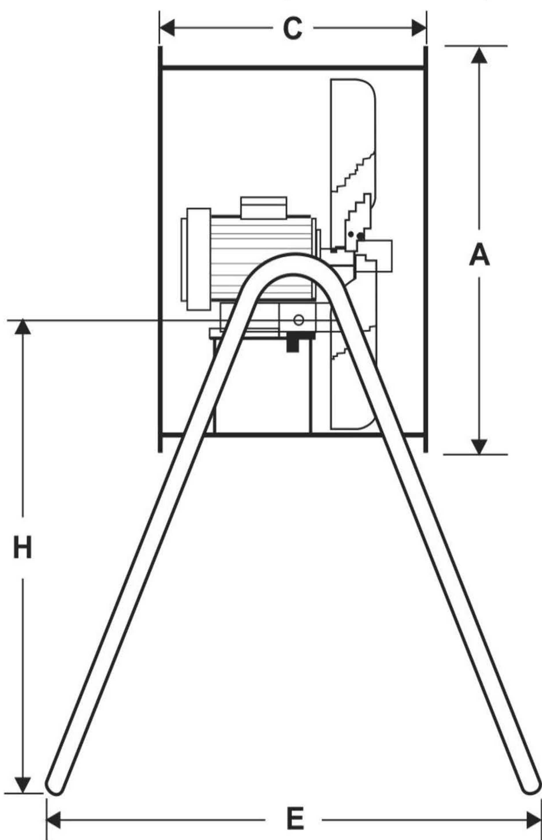
Vista Lateral (Side View)
