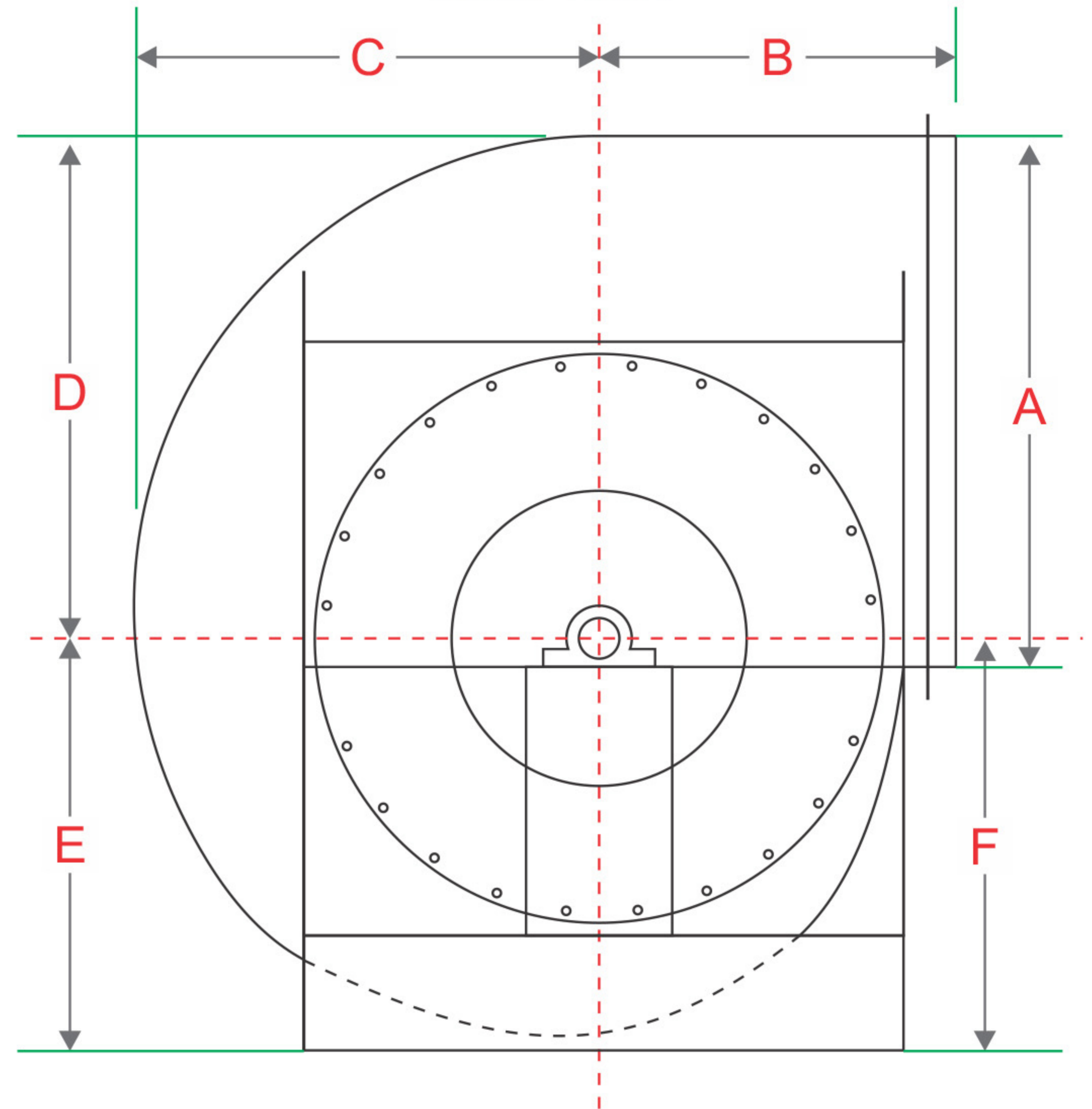
Vista lateral Side view
