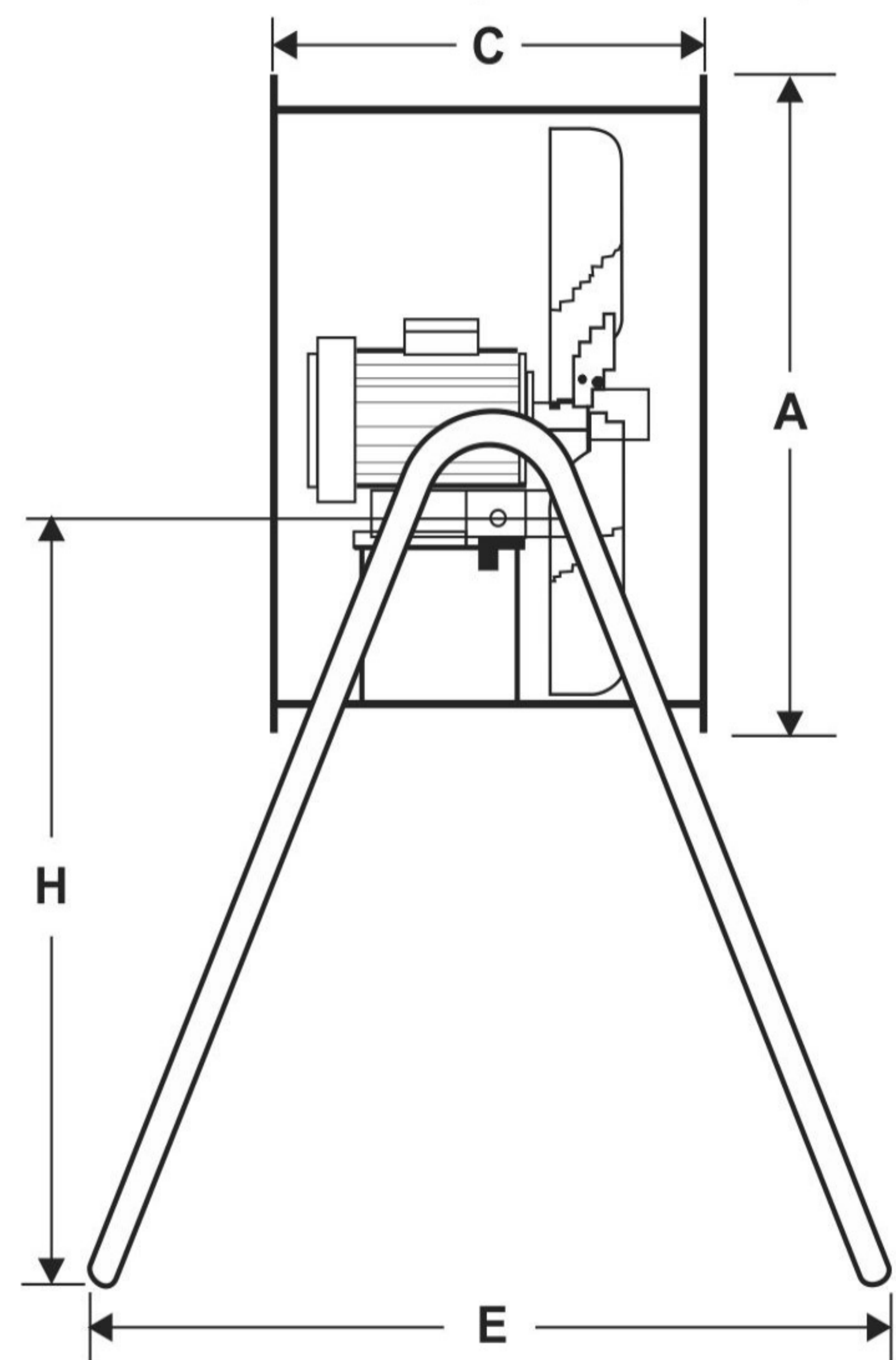
Vista Lateral (Side View)
