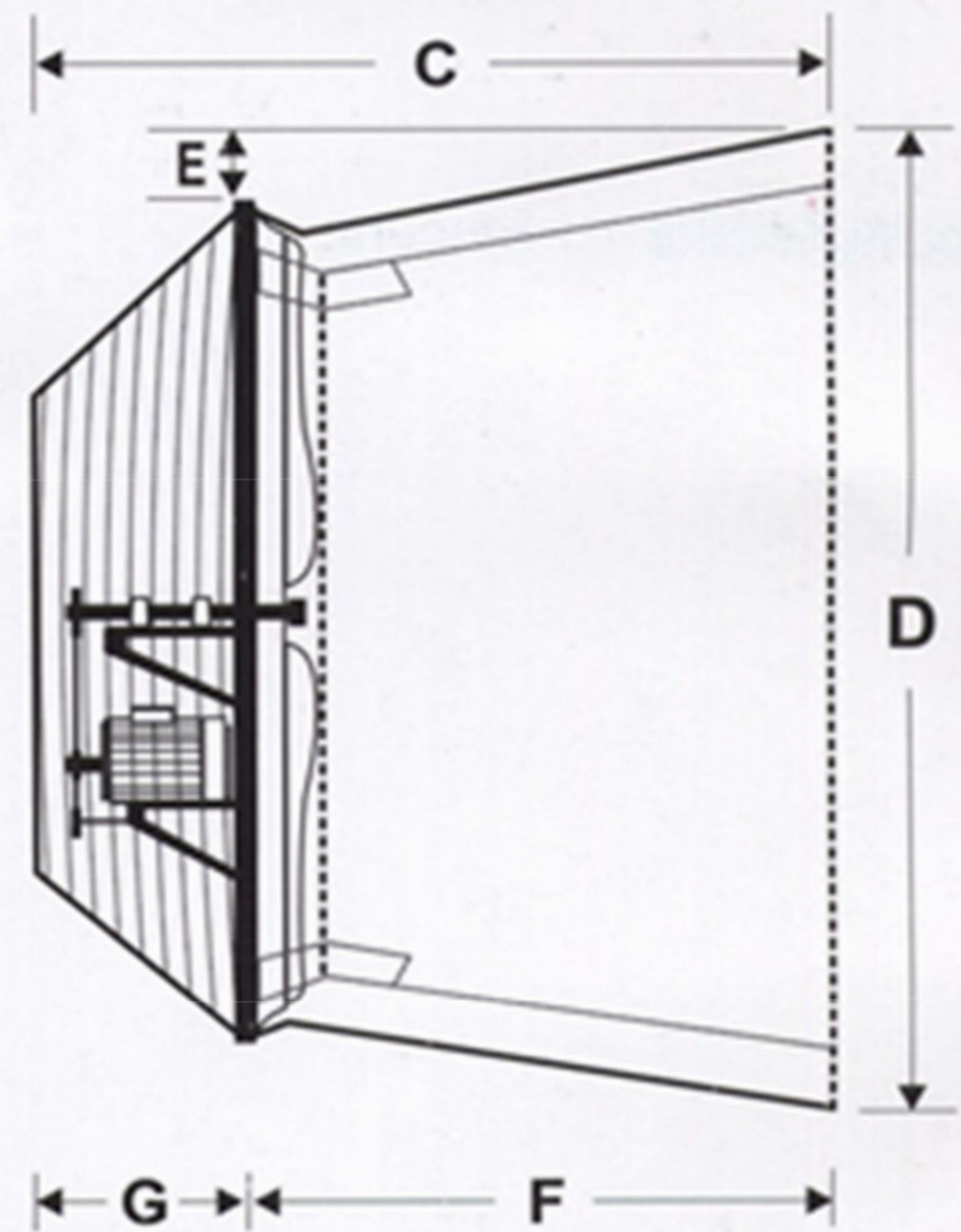
Vista Lateral (Side View)
